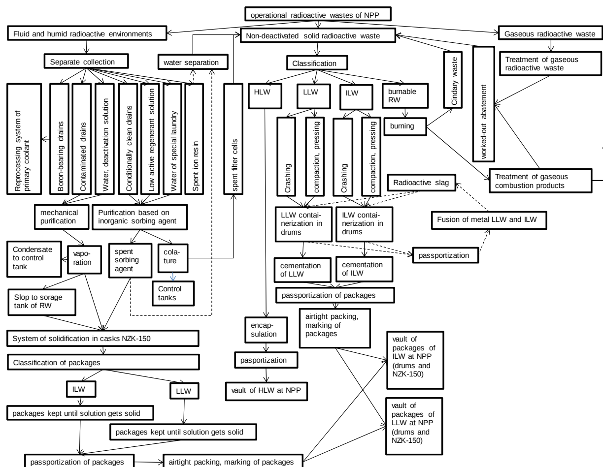
FIG. 7. General scheme of AES-2006 operational radioactive waste handling.
