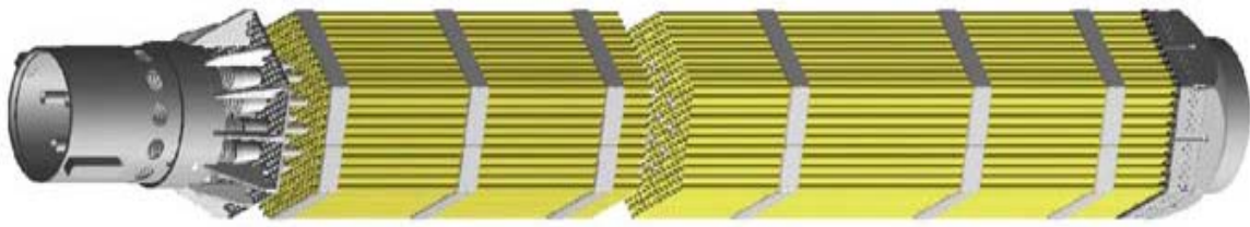
FIG. 19. VVER-1000 fuel assembly of TVS-2M type (figure from Ref. [122]).
