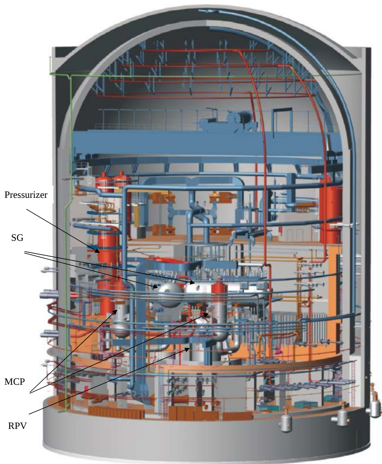
FIG. 18. AES-2006 general layout of reactor building (picture taken from Ref. [123]).
