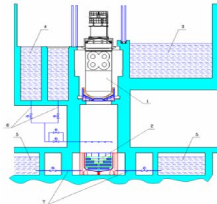
FIG. 17. Water supply to core catcher in case of location of tanks-pits inside containment (AES-2006 design) (reproduced from [123]).
