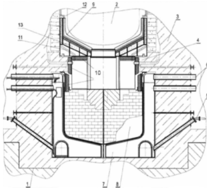
FIG. 16. Core catcher design of AES-2006 [146].
