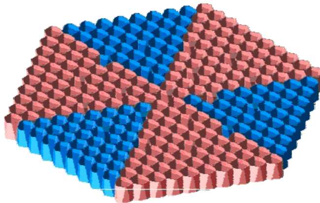
FIG. 10. Spacer of 'sector' coolant mixing type designed for AES-2006 [122].
