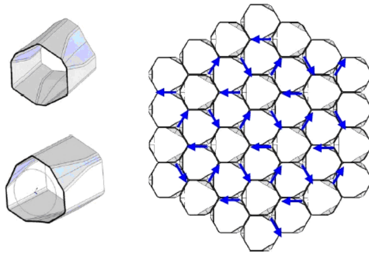
FIG. 9. Spacer cells and part of coolant mixing spacer of 'cyclone' type designed for AES-2006 (Ref. [122]).
