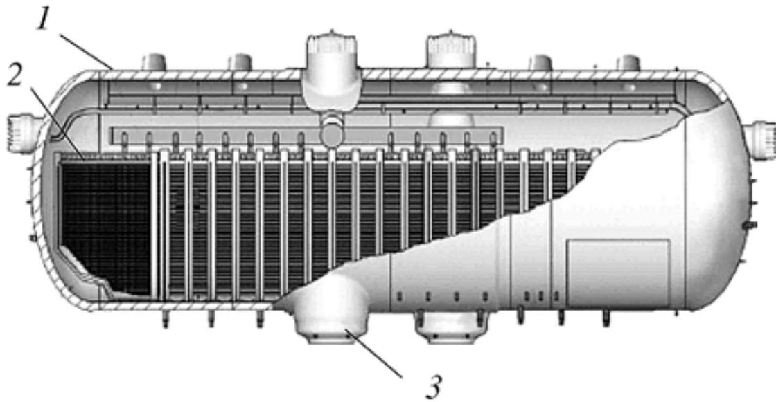
FIG. 20. PGV-1000MK steam generator: 1) housing; 2) tube bank; 3) coolant inflow and outflow stub pipes (figure from Ref. [154]).
