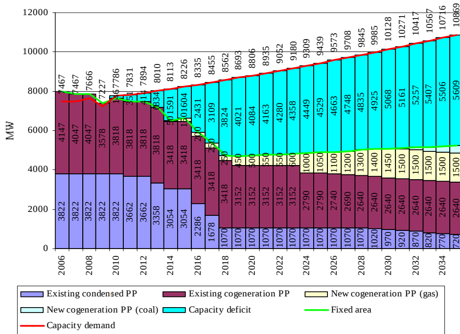
FIG. 4. Deficit of energy system capacity.
