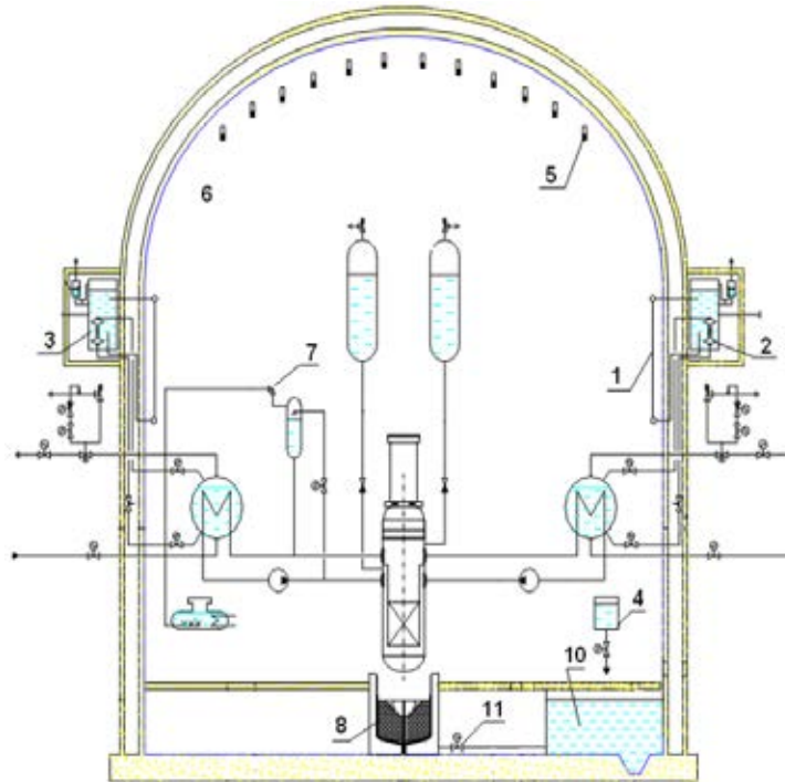
FIG. 13. Overview of BDBA systems of the AES-2006 reactor (reproduced from [123]).
