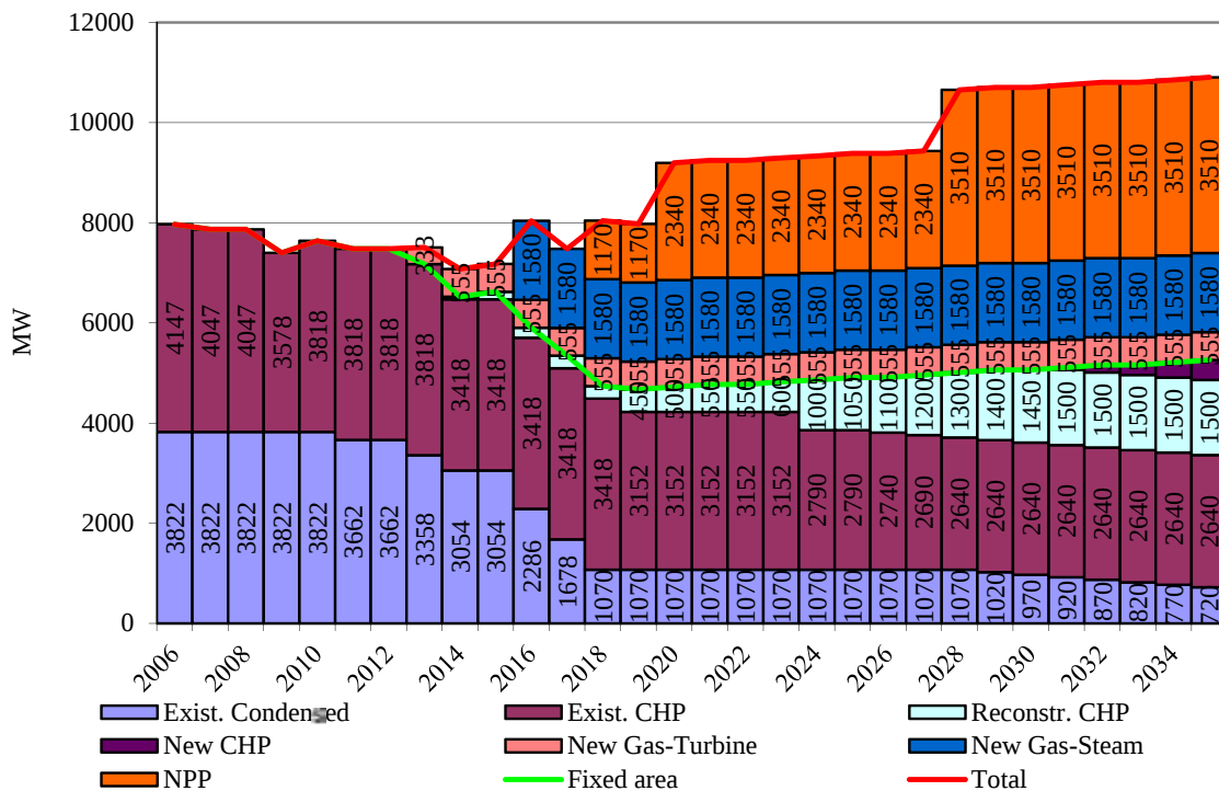
FIG. 5. Structure of electricity system for nuclear scenario.
