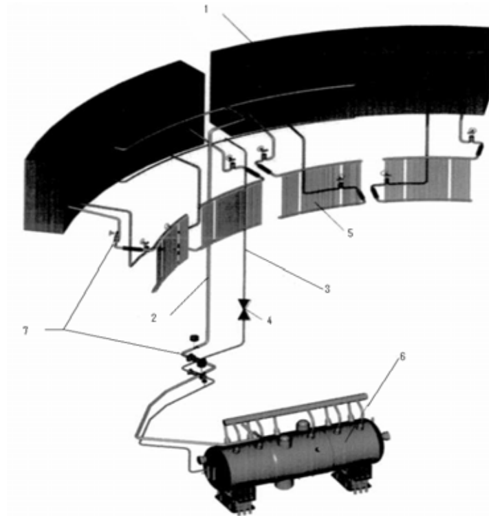
FIG. 14. Passive heat removal system via steam generators (PHRS-SG) of the AES-2006 design (reproduced from [123]).
