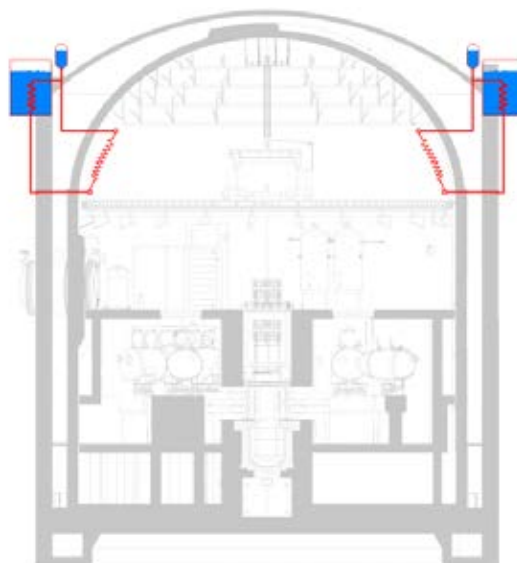
FIG. 15. Passive containment heat removal system (PHRS-C) in AES-2006 design (reproduced from [123]).
