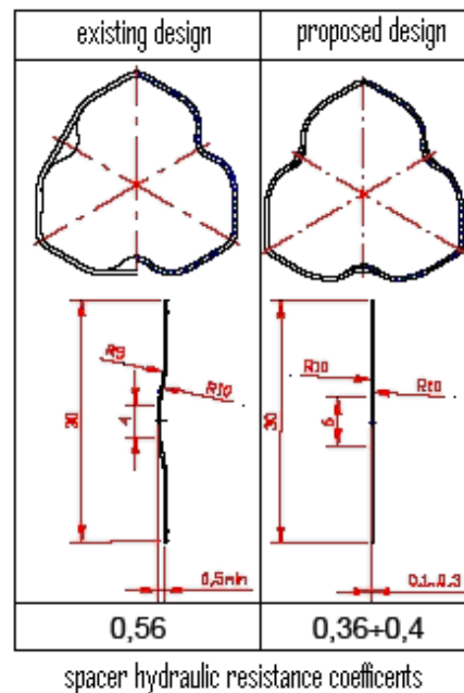
FIG. 8. Existing design of spacer cells for assemblies (TVS-2, TVS-2M) used in V-320 and proposed design of cells for assemblies in AES-2006 (Ref. [122]).
