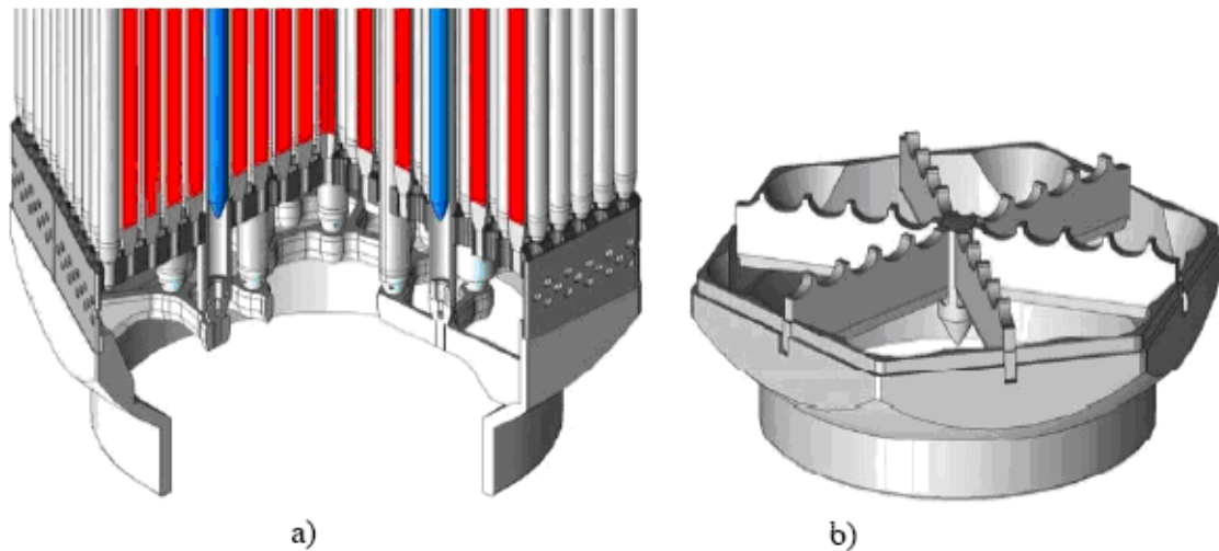
FIG. 12. Lower nozzles of fuel assemblies: (a) – new AES-2006 design with long guide tubes (control rods are blue, red are the fuel rods); (b) – existing nozzle design (TVS-2M, bottom spacer, fuel rods and guide tubes are not shown) has no contact with guide tubes [122].
