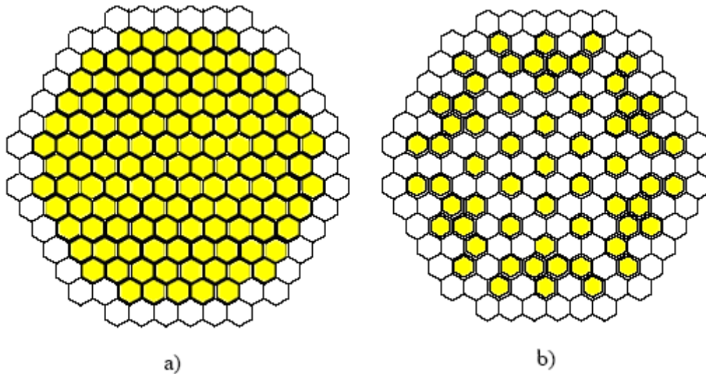
FIG. 11. Position and number of control rods (cells colored yellow) in reactor core of AES-2006 (a) and VVER-1000 (b) [122].
