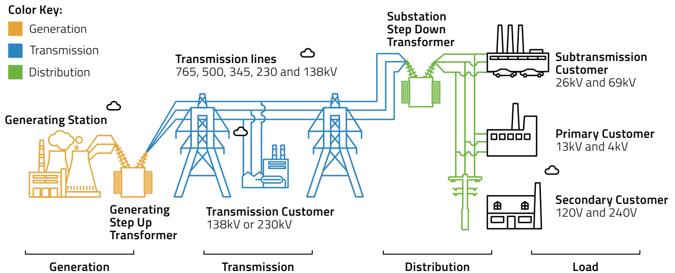
Figure 8.1. Electricity system
