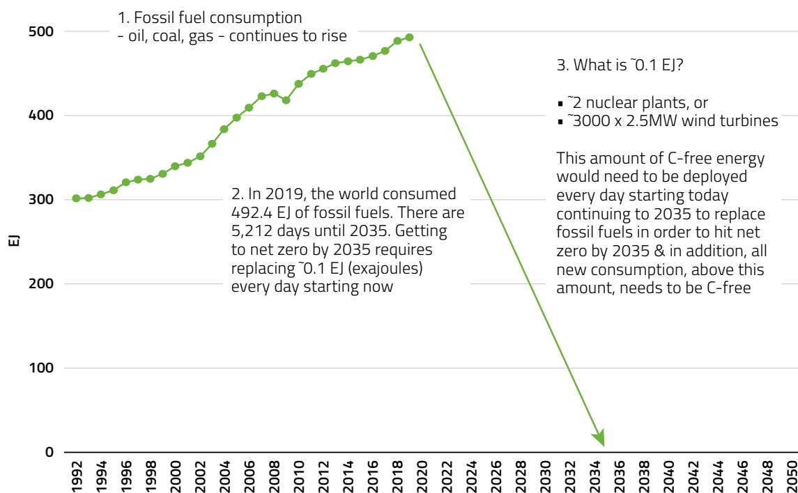
Figure 1.16. Global Fossil Fuel Consumption
