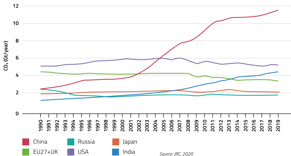
Figure 4.5. Fossil CO 2 emissions of the major emitting economies.
