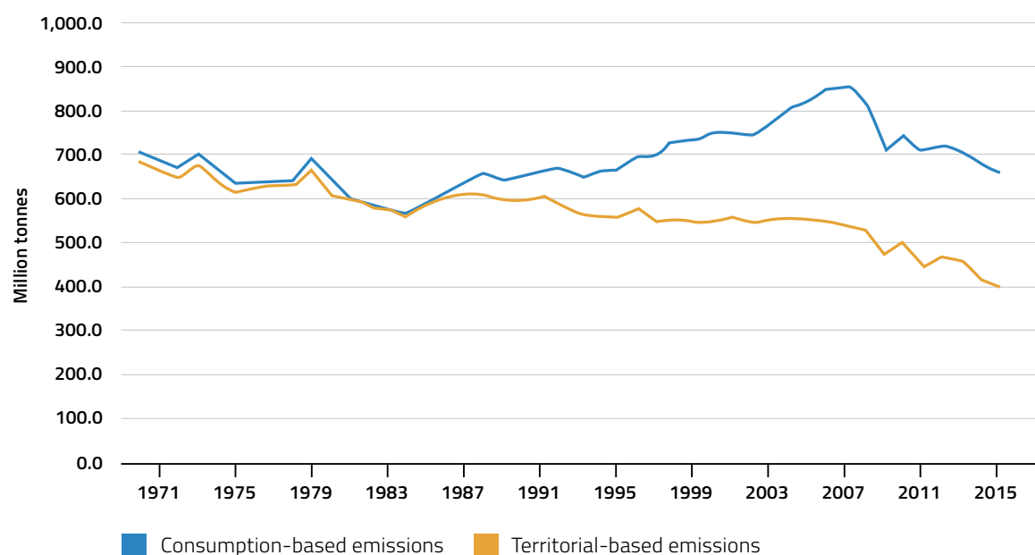
Figure 4.18. Decoupling of GDP per head from CO 2 emissions seems to have happened at the expense of outsourcing manufacturing. 265
